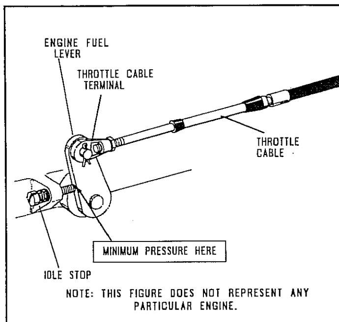
FIGURE 6 THROTTLE CONNECTION
